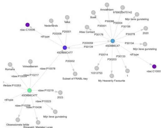
figure 1 Network visualization of the example.
